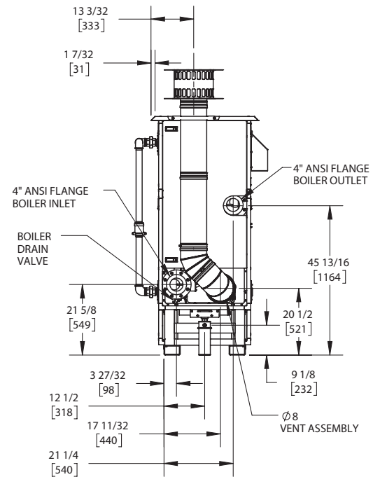
REAR VIEW ASUB-36_E
