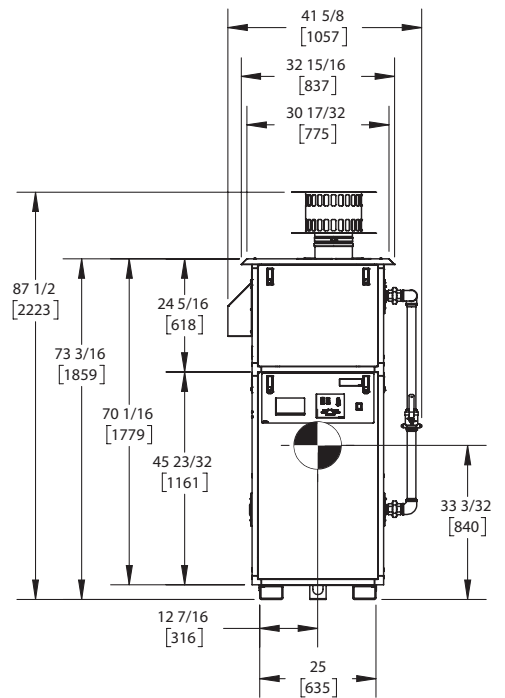
FRONT VIEW ASUB-36_E
